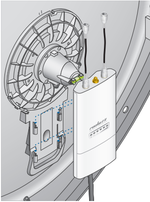
Mounting on a Dish Antenna
