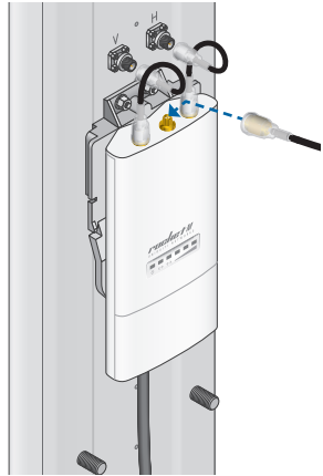
Connecting the GPS Patch Antenna
