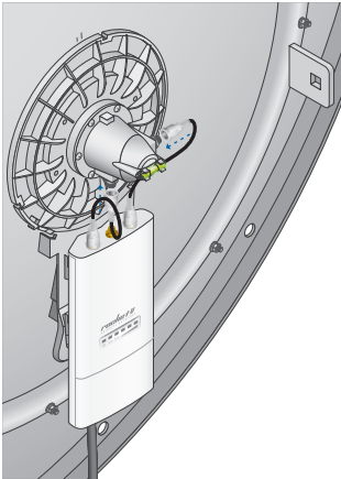
Connecting to a Dish Antenna
