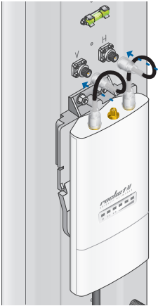
Connecting to a Sector Antenna
