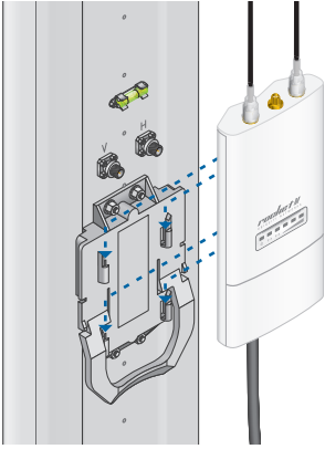
Mounting on a Sector Antenna
