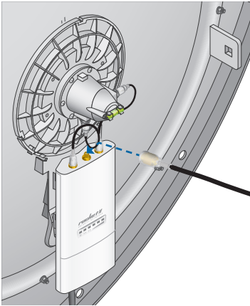
Connecting the GPS Patch Antenna
